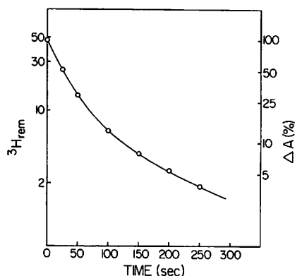
FIGURE 3: Computed kinetic progress curve for a hypothetical folding reaction without intermediates but with two unfolded forms which refold at different rates. The two unfolded species are present in a 20:80 ratio with time constants for folding of \tau = 150 s and \tau = 30 s, respectively. Folding is measured by tyrosine absorbance and by protection of amide protons against exchange. Both unfolded species are assumed to have the same extinction coefficient in measurements of tyrosine absorbance. (—) The normalized curve calculated for absorbance changes ( \Delta A ). (O) Calculated number of protons stably trapped per RNase A molecule ( {}^3H_{\text{rem}} ). The calculations show that when there are multiple unfolded species present initially, which have different rates of folding, then the kinetic progress curves become complex but the normalized folding kinetics are still superimposable [see the analysis of the kinetic ratio test by Labhardt & Baldwin (1979)].
