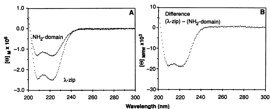
Fig. 1. Circular dichroism studies (11). (A) Spectra of 10 \mu M solutions of purified \lambda -zip protein and the NH 2 -terminal domain of \lambda repressor (residues 1 to 102). [\theta]_M , molar ellipticity. (B) Difference spectrum of residues 103 to 165 of \lambda -zip was calculated by subtracting the spectrum of the NH 2 -terminal domain (residues 1 to 102) from the spectrum of \lambda -zip, and converting the difference to units of mean residue weight ellipticity [\theta]_{MRW} .
