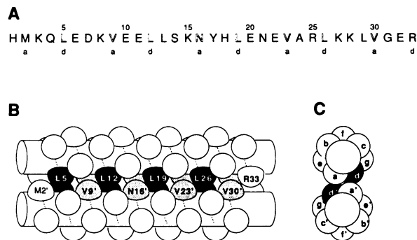
Fig. 2. The leucine zipper of GCN4 modeled as a coiled coil (2). (A) Sequence of the GCN4 leucine zipper. The a and d positions that form the core of the dimer interface are shown in outline. (B) Side-view depiction of parallel \alpha -helices in the leucine zipper dimer. The a (stippled) and d (black) positions in the dimer interface that have been studied here are indicated. (C) End view of structure shown in (B). Positions around the helical wheel are labeled a through g . The d position, which is usually leucine, is shown in black.
